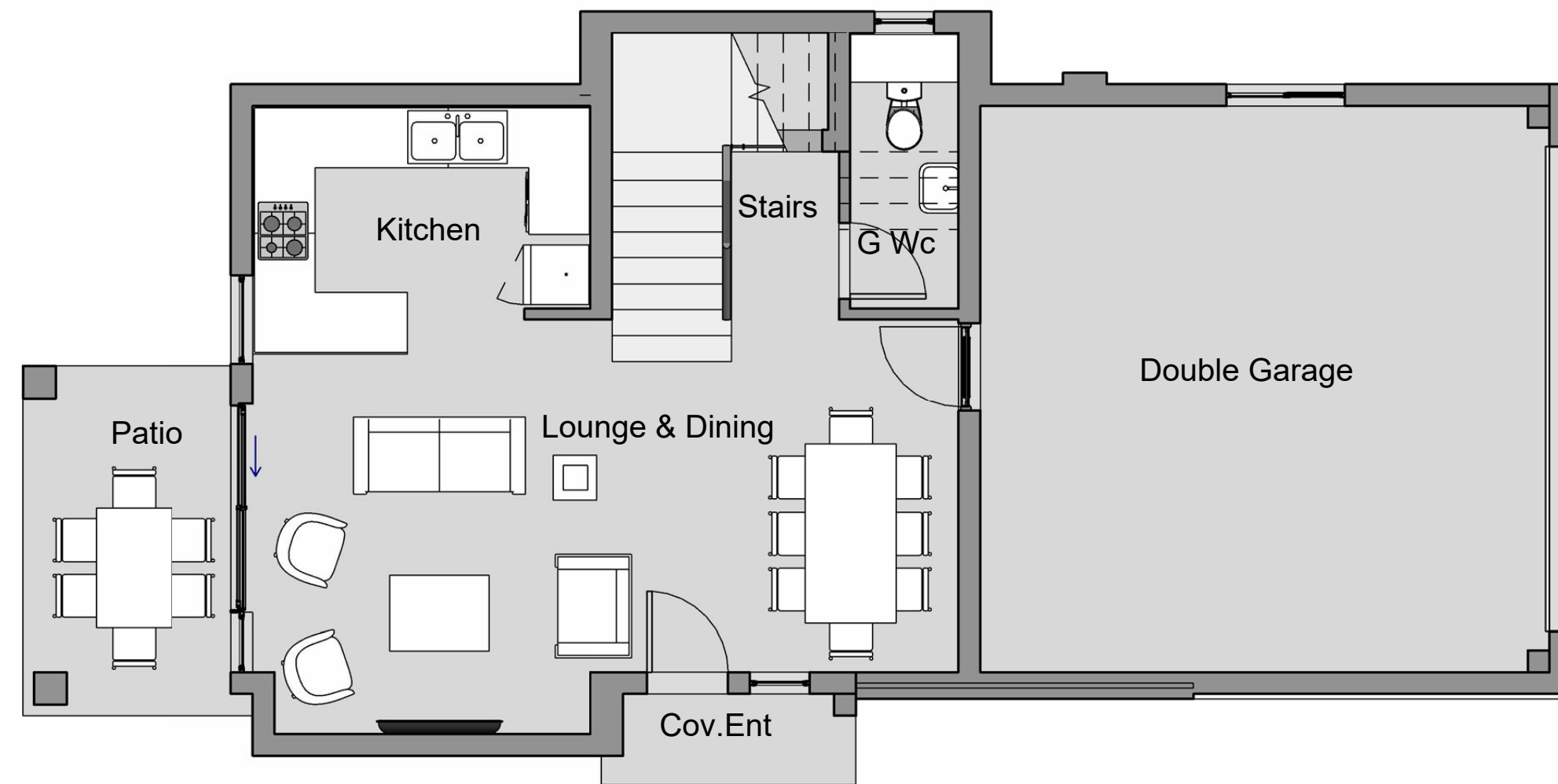
GROUND FLOOR
