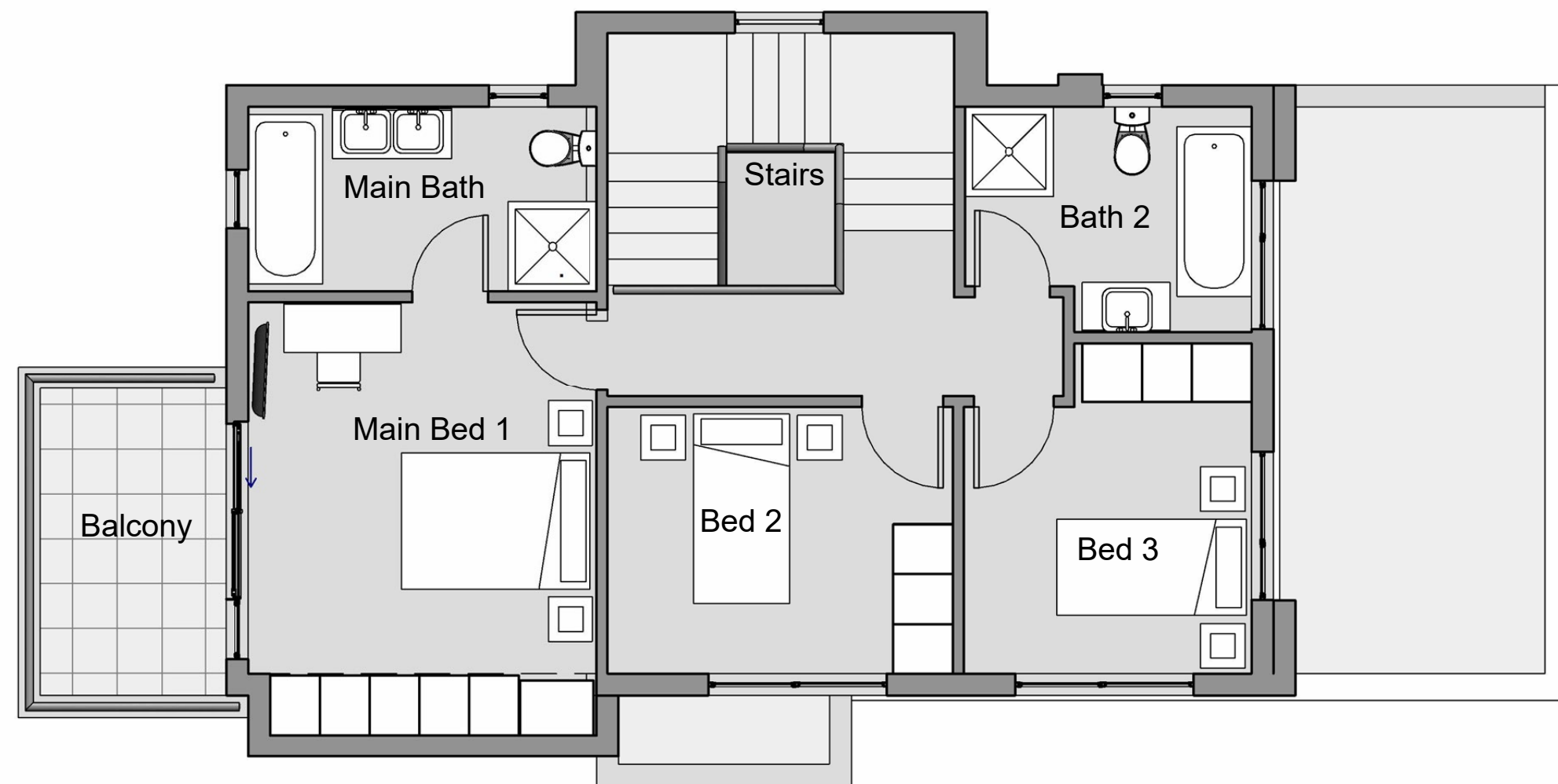
FIRST FLOOR
