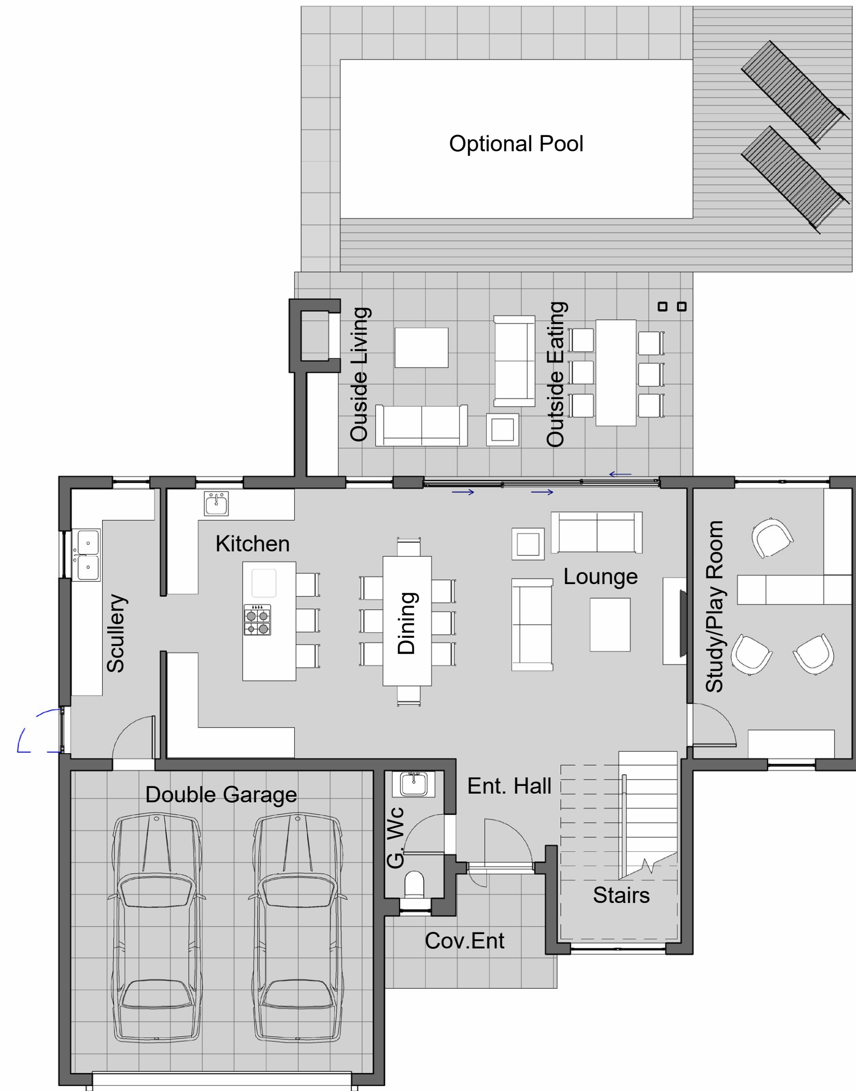
GROUND FLOOR
