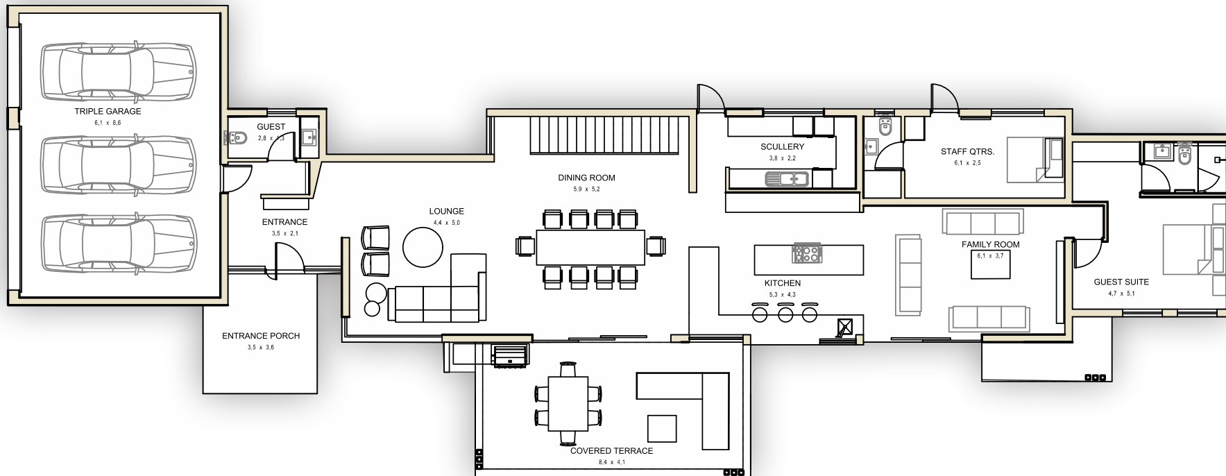
Ground floor plan - NTS
