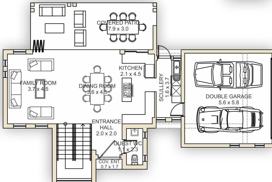
First floor plan - NTS
