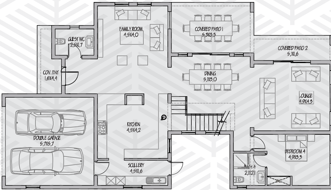
ground floor plan - not to scale
