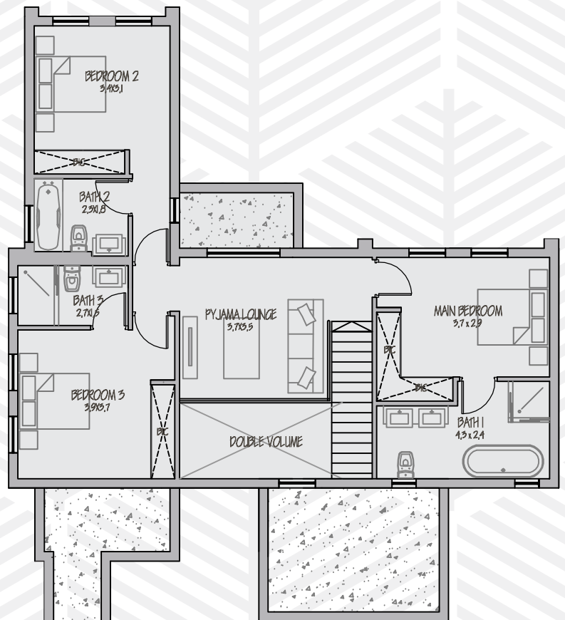
first floor plan - not to scale
