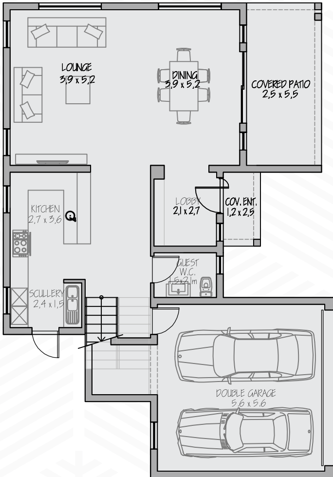
ground floor plan - not to scale
